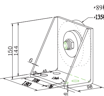
YS-181EA YS-131EA
